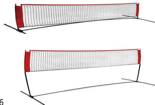
MS-006 1. Size: 10 ft x 3- 5 ft 2. Frame: Φ25*1.0mm steel tube with 12.7mm fiberglass pole 3. Net: PE 30-ply knotted 4.5cm 4. Bag: 420D Oxford fabric carry bag
