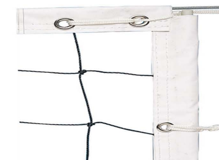
VB-009 Indoor & Outdoor Volleyball Net 1. Size: 9.5m x 1m 2. Net: 3.0mm PE 10cm twisted knotted net 3. Top: 0.6mm white PVC band x 2" 4. Sides 0.6mm white PVC band x 2.5" 5. Bottom: 0.6mm white PVC band x 2" 6. With a 6mm steel cable on top and 5mm steel cable at bottom 7. Equipped with 2 dia 11mm fibreglass poles 8. Packing: 1 set in PE bag, 4 sets in carton
