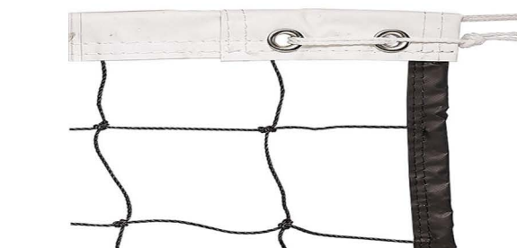
VB-007 Volleyball Practice Net 1. Size: 9.5m x 1m 2. Net: 1.5mm PE 10cm twisted knotted net 3. Top: 0.35mm colored PVC band x 1.5" 4. Sides & Bottom: Overlocked 5. With a 6mm PE rope on top for hanging up 6. Packing: 1 set in PE bag, 12 sets in carton
