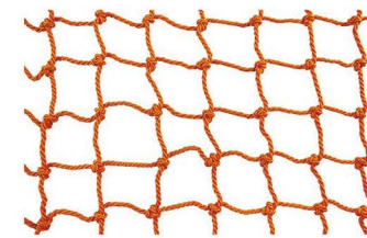
Polyester & Nylon Knotted Net 1. Twine Diameter: 210D 2. Number of ply: 6ply-300ply 3. Mesh size: 12mm-500mm 4. Application: Sports Net, Protection Net, Safety Net, Agriculture Net, Fishing Net
