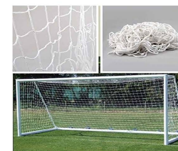
FB-023 Metal Soccer Goal 1. Size: 1.2x0.8, 1.5x1, 1.8x1.2, 3x1.2x2, 5x1.4x2m 2. Net: Mesh 4, 4.5, 5, 5.5", twine diameter 1.5mm to 6mm, polyester/nylon 3. Frame: Tube thick vary from 0.8mm to 2.5mm, dia 32, 48, 60, 76, 90, 114mm 4. Knotless/ knotted, braided/twisted, square/hexagon shape
