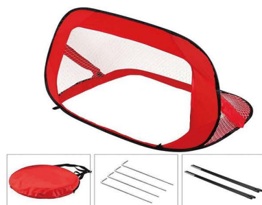
FB-014 Portable Pop-up Goal 1. Size: 120 x 80 x 80cm 2. Net: Polyester knotless 1.75" mesh & 210D binding 3. Frame: 2mm thick steel wire 4. Packing: 1 pair in bag, 5 pairs in carton
