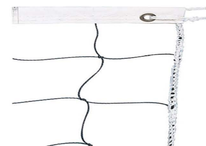
VB-008 Volleyball Net 1. Size: 9.5m x 1m 2. Net: 1.8mm PE 10cm twisted knotted net 3. Top: 0.35mm colored PVC band x 1.5" 4. Sides & Bottom: Overlocked 5. With a 3mm steel cable on top for hanging up 6. Packing: 1 set in PE bag, 12 sets in carton
