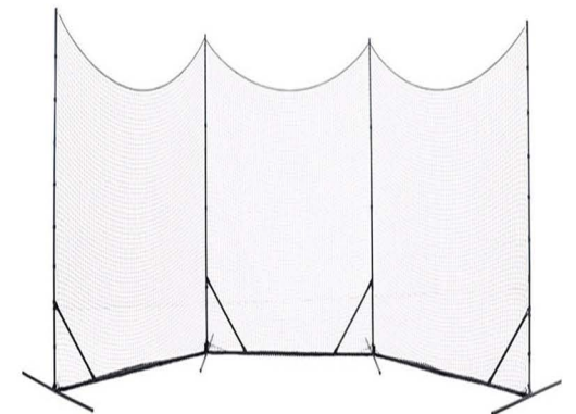
LG-010 Lacrosse Portable Backstop 1. Size: 12 x 9' 2. Material: UV metal tube, polyester net
