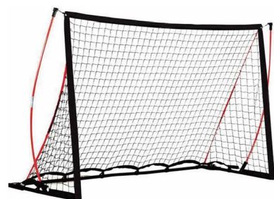
FB-004 6' x 4' Flexpro Portable Soccer Goal 1. Size: 6 x 4', 6 x 4', 7 x 5', 12 x 6' 2. Net: Polyester 5 ply 4" 3. Frame: 1" dia tube, 12.7mm flex tension poles
