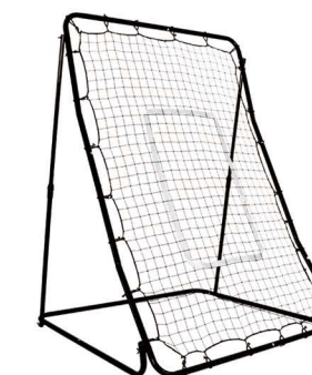
BS-023 Adjustable Baseball and Softball Rebounder PitchBack Net 1. Size: 5.33 x 3.67' (64 x 44 inch) 2. Net: 30 ply PE knotted net 3. Frame: 1-1/4" diameter steel tube
