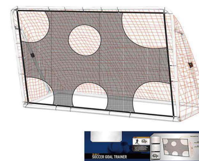
FB-021 Soccer Goal with Target 1. Size: 7 x 5 x 3' 2. Net: 4" Polyester knotless net 3. Frame: Steel pole Dia 1"
