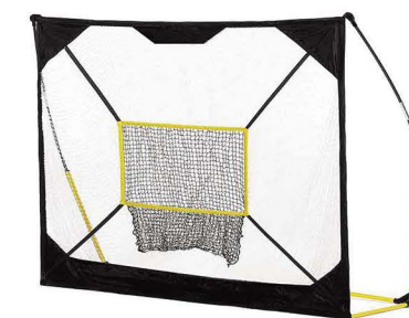
BS-011 Quickstar Baseball Net 1. Size: 5x5', 7x7' 2. Net: 1" dia powder tubing with 1.75" heavy duty net 3. Frame: Composite steel & Tension-Tite fiberglass
