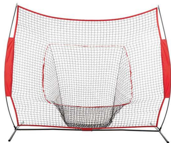
BS-001 7x7' Baseball & Softball Practice Hitting Net 1. Net: Polyester 7 ply 1.75" with 600D oxford fabric edge 2. Frame: Φ25*1.0mm Iron pipe, 12.7mm fiberglass poles
